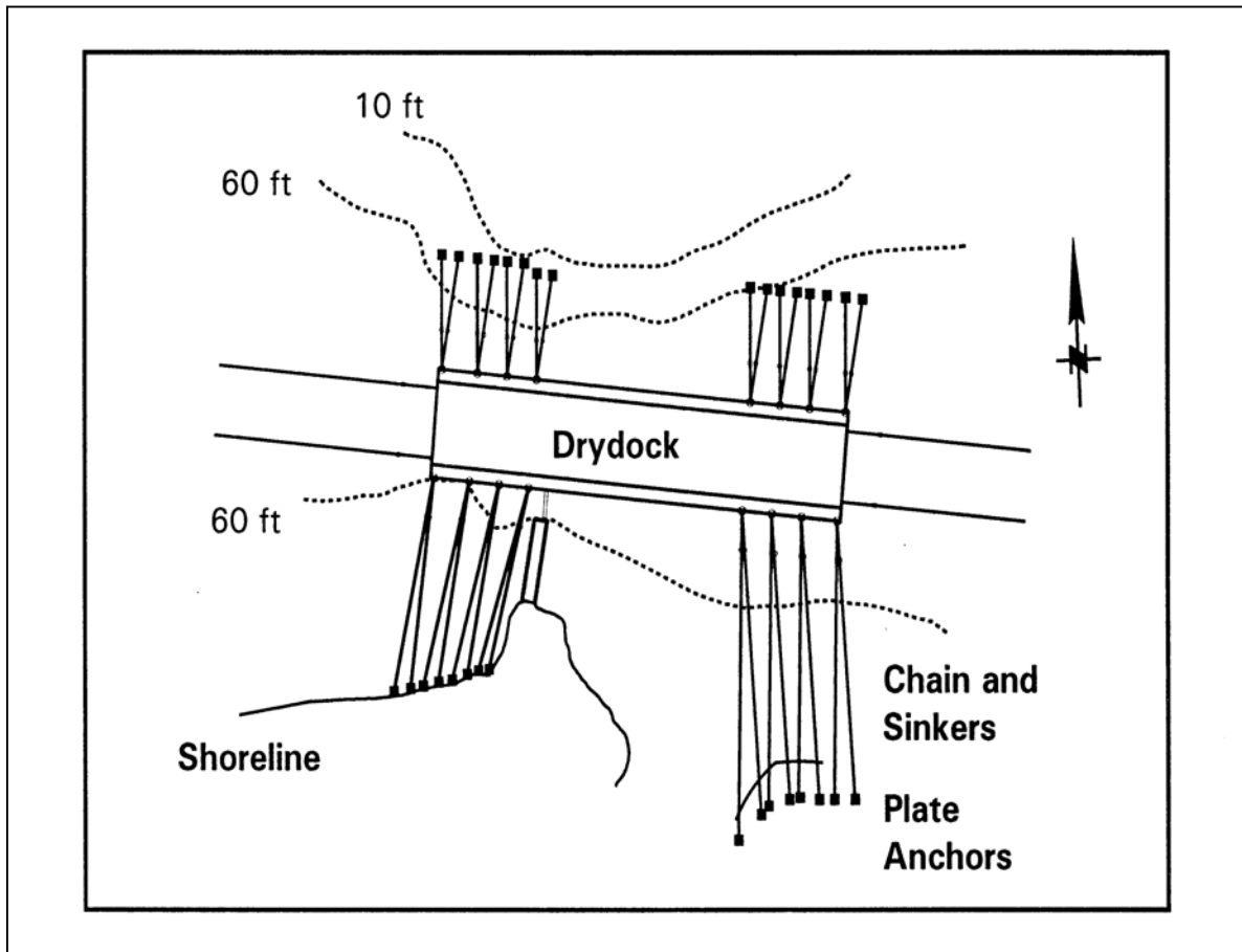
Figure 2-11. Spread Mooring
