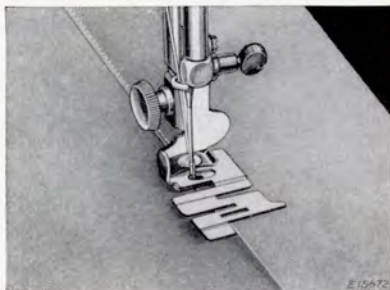
FIG. 48. MAKING A WIDE HEM
