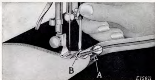
FIG. 38. ADJUSTING THE BINDER
