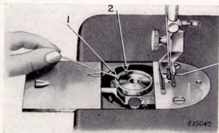
FIG. 8. THREADING THE BOBBIN CASE
