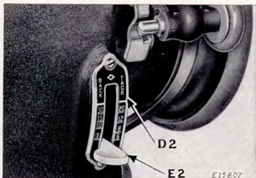
FIG. 16. STITCH REGULATOR
