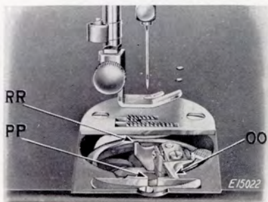
FIG. 25. SHOWING THE BOBBIN CASE POSITION BRACKET
