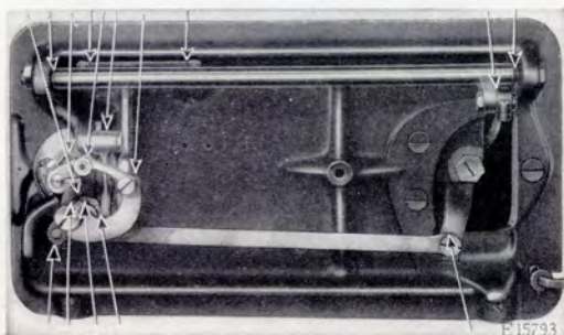
FIG. 20. OILING POINTS AT THE BASE OF MACHINE
