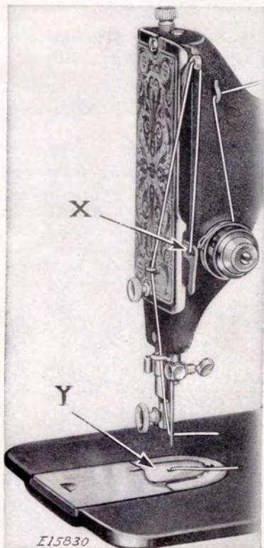
FIG. 61. MACHINE THREADED FOR EMBROIDERY AND DARNING
