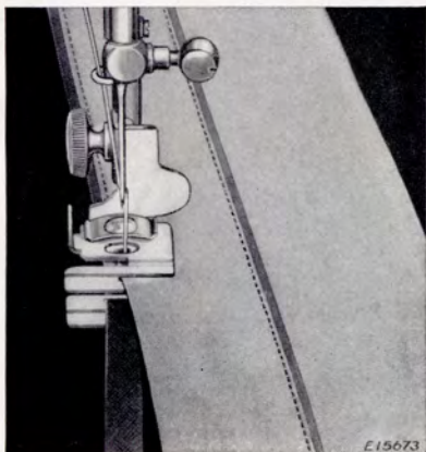
FIG. 46. PIPING WITH THE EDGE-STITCHER
