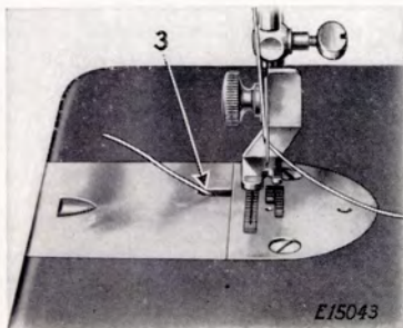
FIG. 10. UNDER THREADING COMPLETED
