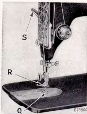
FIG. 3. FRONT VIEW OF THE MACHINE
