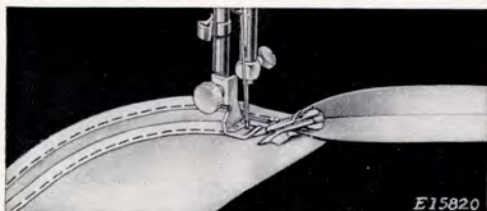
FIG. 42. APPLYING FRENCH FOLDS
