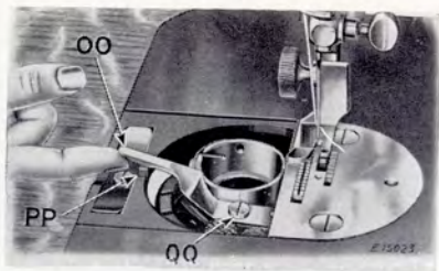
FIG. 23. RAISING THE LATCH
