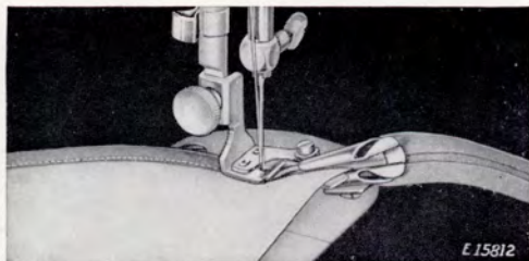
FIG. 39. BINDING AN OUTSIDE CURVE
