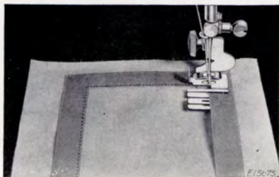
FIG. 47. APPLYING BIAS FOLDS WITH THE EDGE-STITCHER
