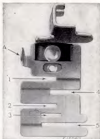
FIG. 43 THE EDGE-STITCHER
