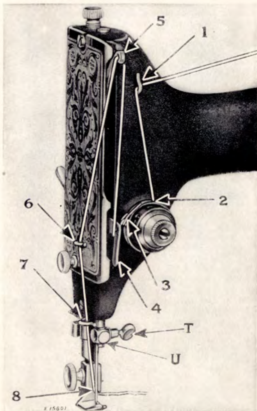
FIG. 11. UPPER THREADING
