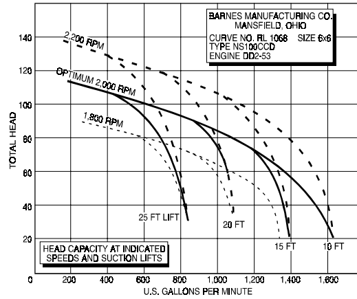
Figure 7-4B. Performance Curve, 6-inch Diesel Pump.
