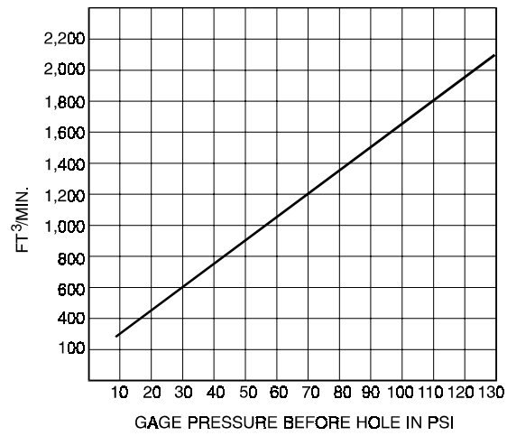
Figure 7-1. Air Discharge Through a One-Inch-Hole.
