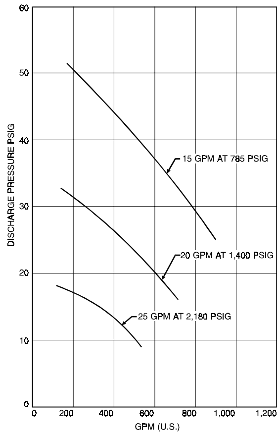
Figure 7-41. Performance Curve, 4" Hydraulic Submersible Pump.
