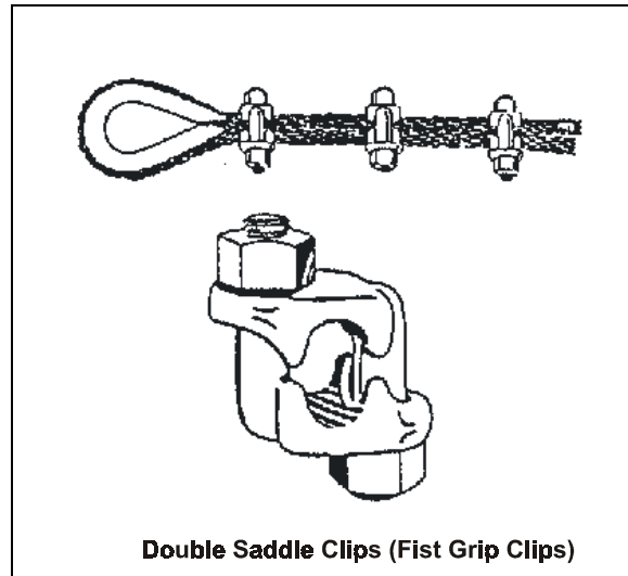
Figure 3-4. Double Saddle Clips (Fist Grip Clips).
