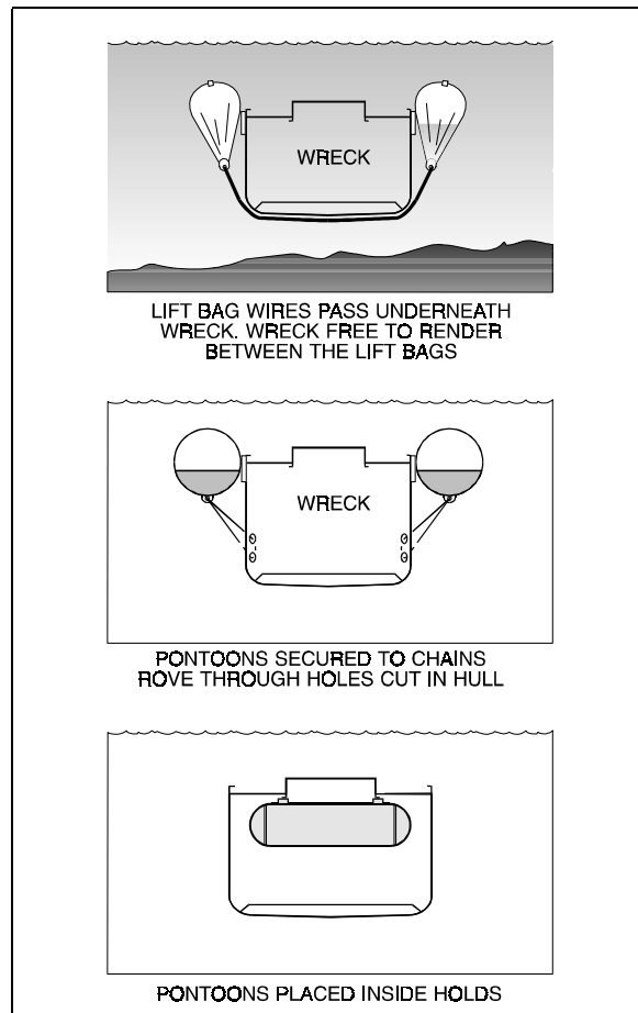
Figure 3-15. Rigging Pontoons and Lift Bags.
