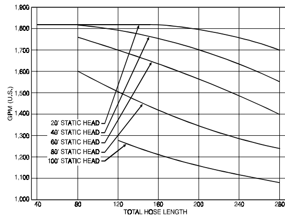
Figure 7-4K. Performance Curve, CCN-150 (Water), CCN-150 Pump (6" Hose).
