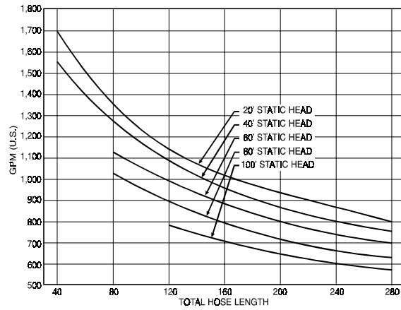
Figure 7-4J. Performance Curve (Water), CCN-150 Pump (4" Hose).
