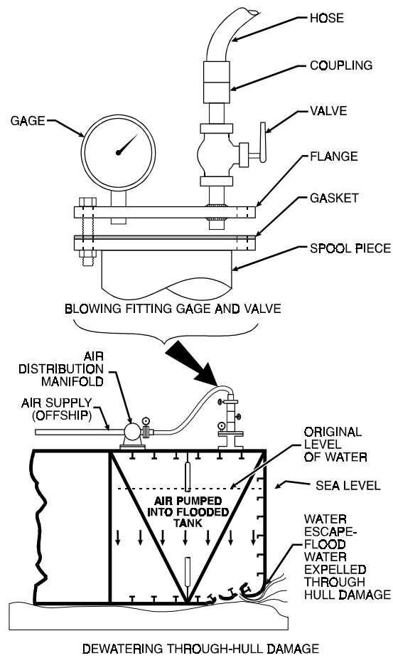
Figure 5-20A. Blowing Techniques.
