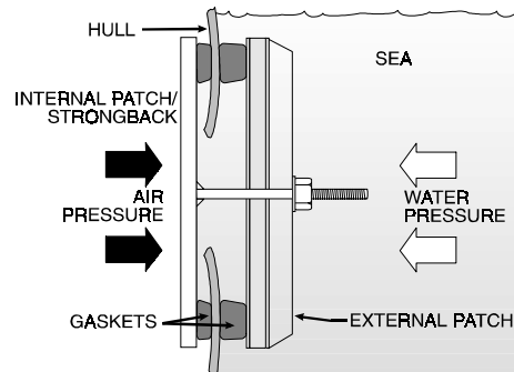
Figure 5-1. Double Patch.
