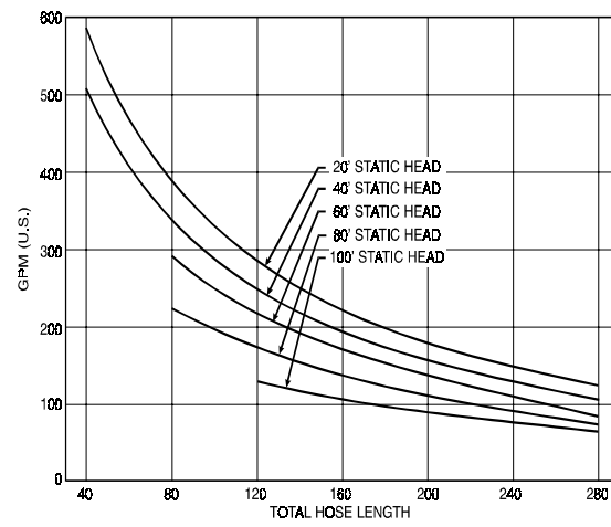
Figure 7-4L. Performance Curve, (Warm #6) CCN-150 Pump (4" Hose).
