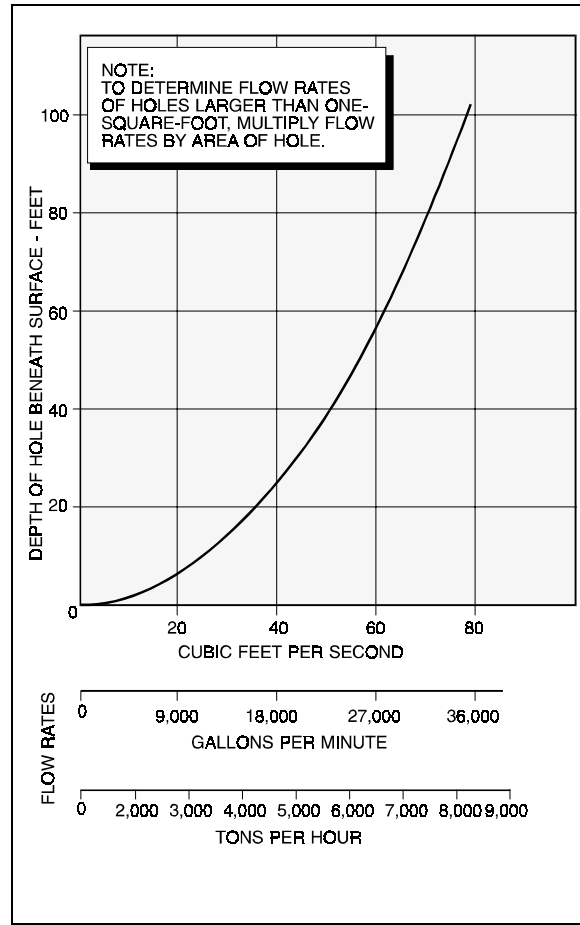
Figure 1-2. Flow Through a One-Square-Foot Hole.
