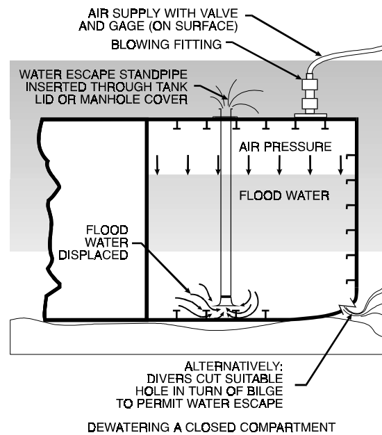
Figure 5-20B. Blowing Techniques.
