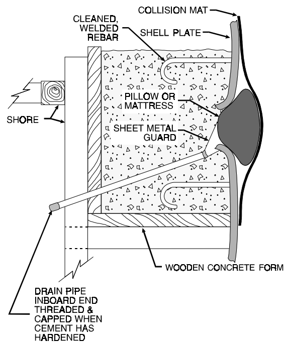
Figure 5-9. Small Concrete Patch.
