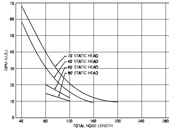
Figure 7-N. Performance Curve, (Cold #6) CCN-150 Pump (4" Hose).
