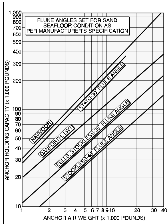
Figure 3-10. Drag Anchor System Holding Capacity in Sand.
