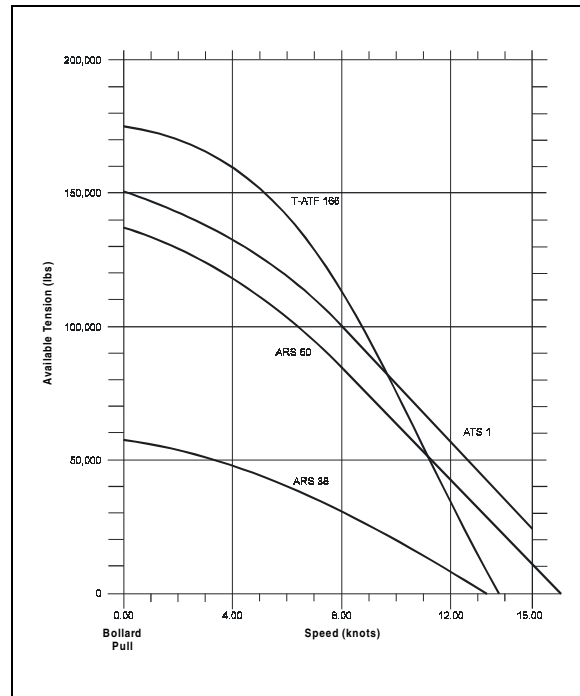
Figure 7-7. Available Tension vs. Ship's Speed for U.S. Navy Towing Ships.
