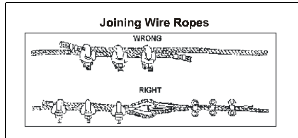
Figure 3-6. Joining Wire Ropes.
