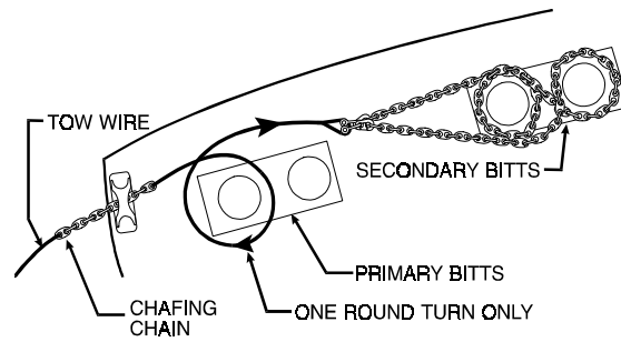
Figure 6-3. Sharing Towing Load Between Bitts.
