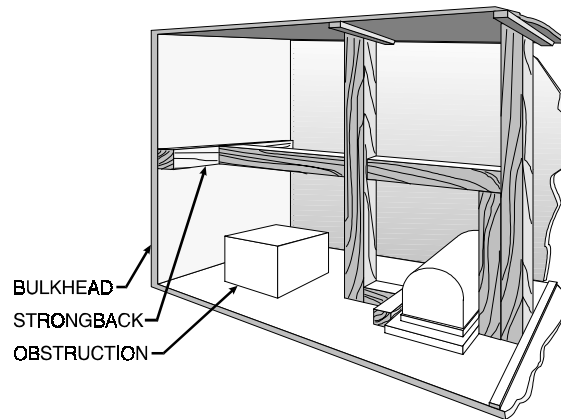
Figure 5-12. Direct Compression Shoring.
