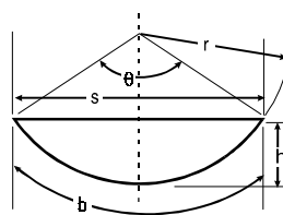
Figure 7-2B. Properties of Plane Surfaces.
