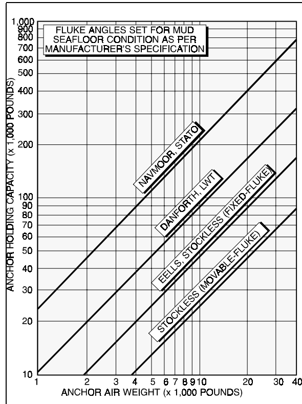
Figure 3-9. Drag Anchor System Holding Capacity in Mud.
