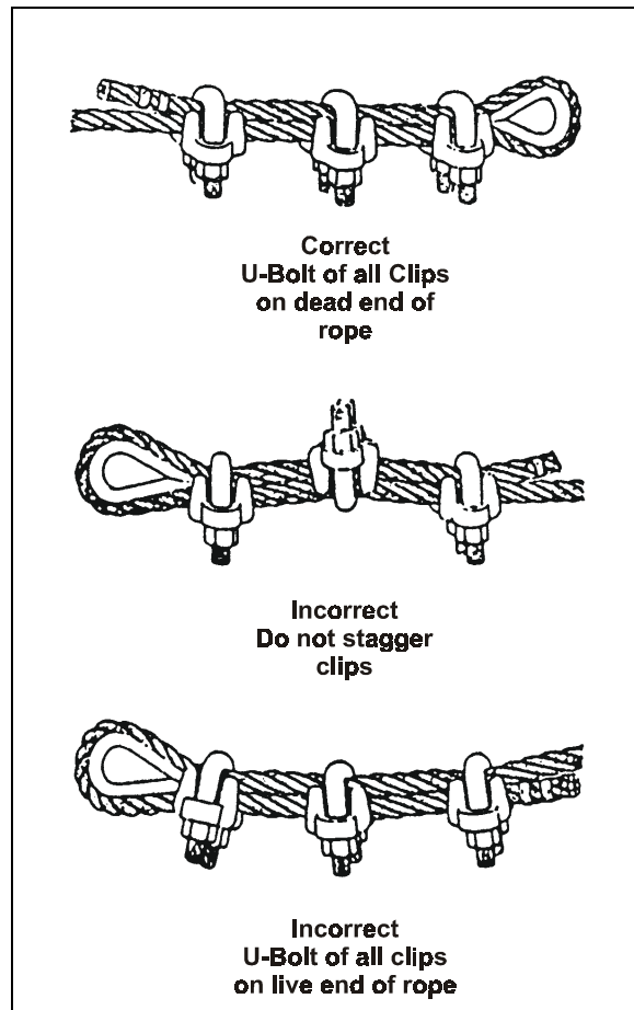
Figure 3-2. Right and Wrong Way of Using Cable Clips.
