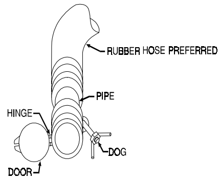
Figure 5-10. Cement Gun.
