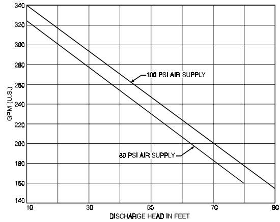
Figure 7-4D. Performance Curve, 2 1/2" Air Submersible Pump.
