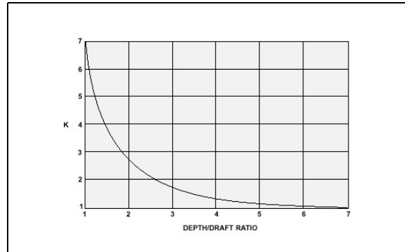
Figure 7-4R. Current Force Depth Correction Factor (K)
