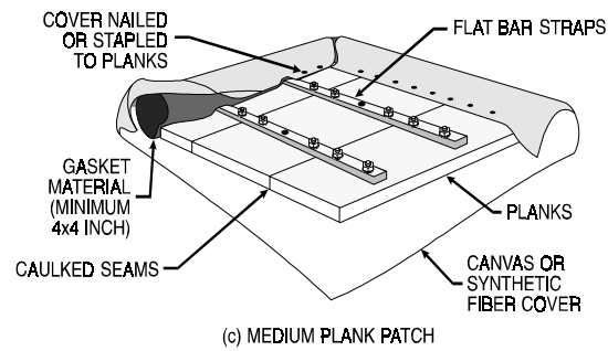
Figure 5-4. Wooden Patch Construction.
