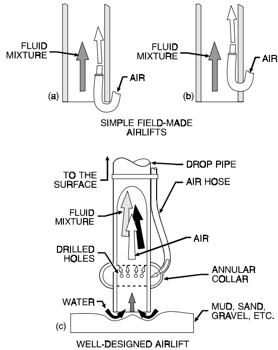
Figure 5-18. Air Lifts.
