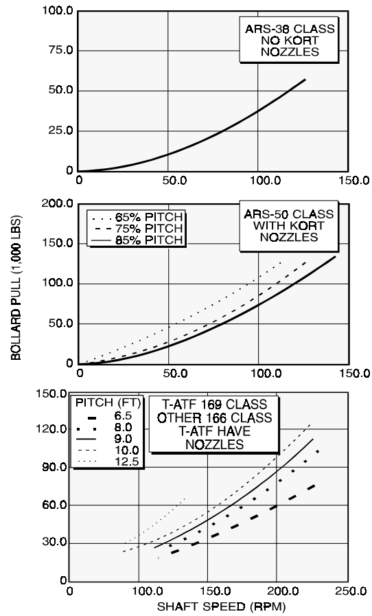
Figure 7-5. Bollard Pull Curves.
