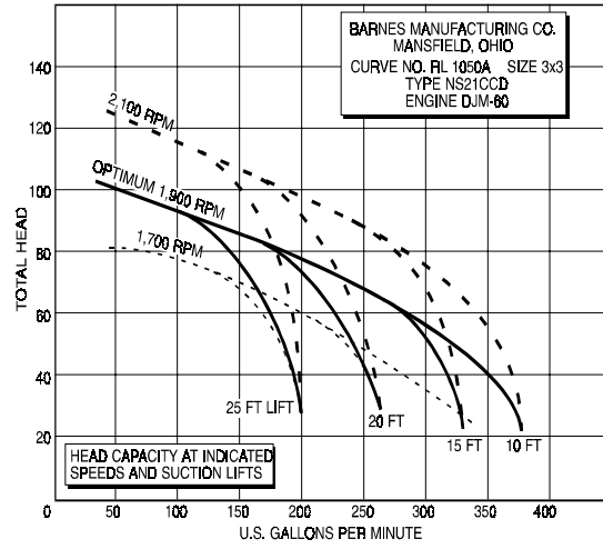
Figure 7-4A. Performance Curve, 3" Diesel Pump.
