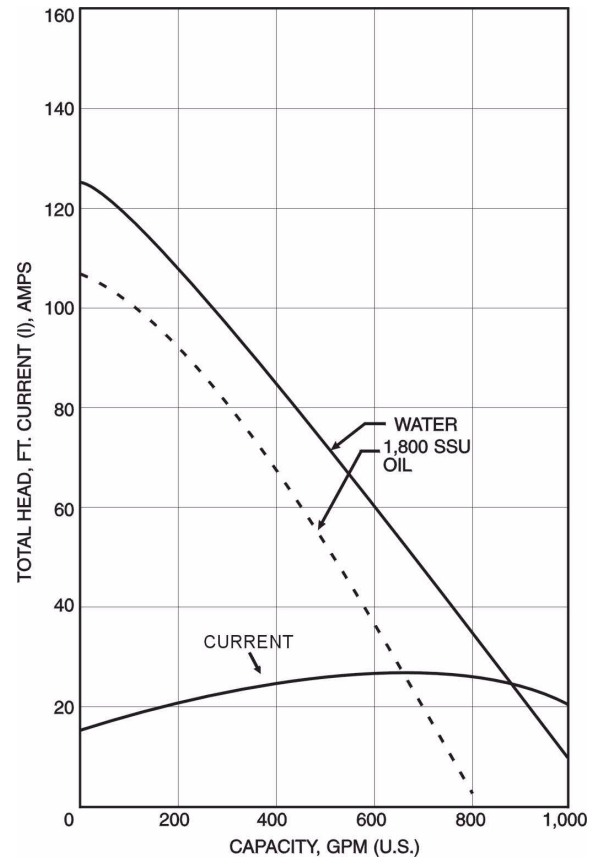
Figure 7-4G. Performance Curve, U.S. Navy 4" Electric Submersible Pump (Impeller No. 4).
