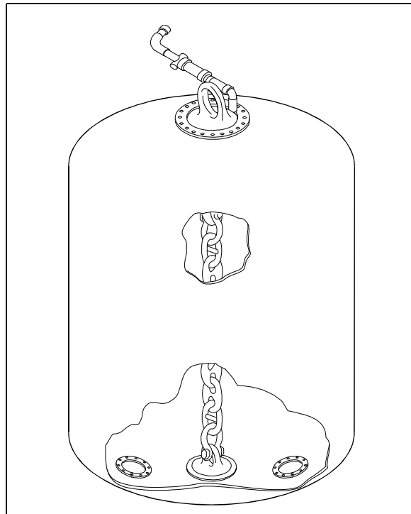
Figure 3-13. 8.4 Ton Inflatable Salvage Pontoon.
