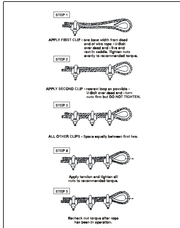
Figure 3-3. Proper Method of Installing Cable Clips.
