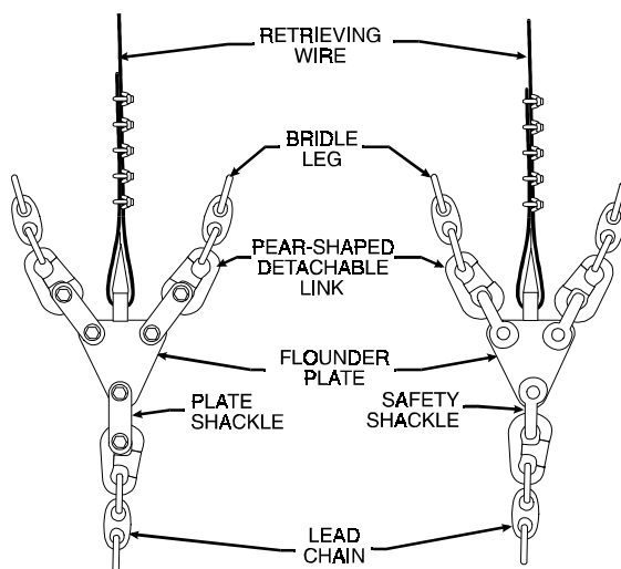
Figure 6-6B. Flounder Plate Connections.
