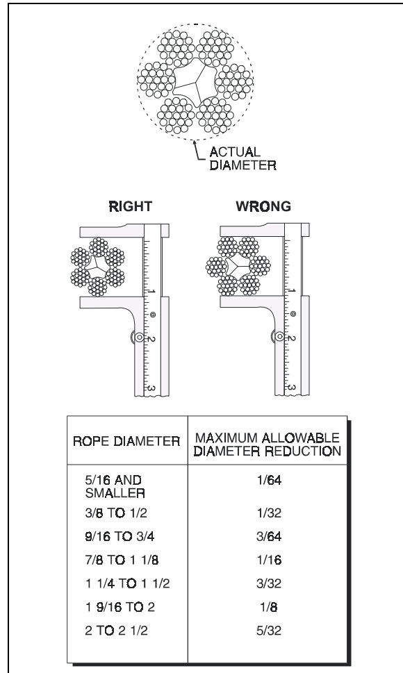
Figure 3-1. Wire Measurement and Reduction Limits.
