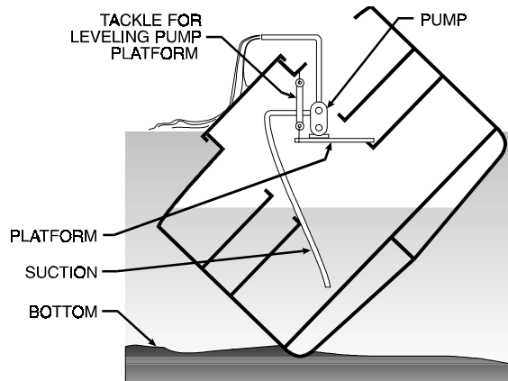
Figure 5-19C. Pumping Arrangements.
