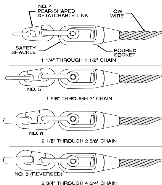
Figure 6-7. Towline Connections.
