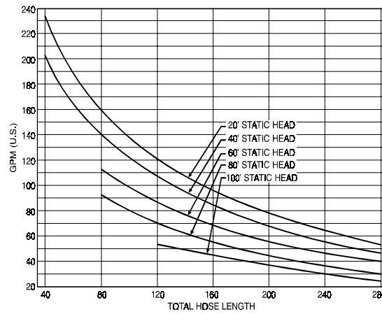
Figure 7-40. Performance Curve, (Cold #6) CCN-150 Pump (6" Hose).
