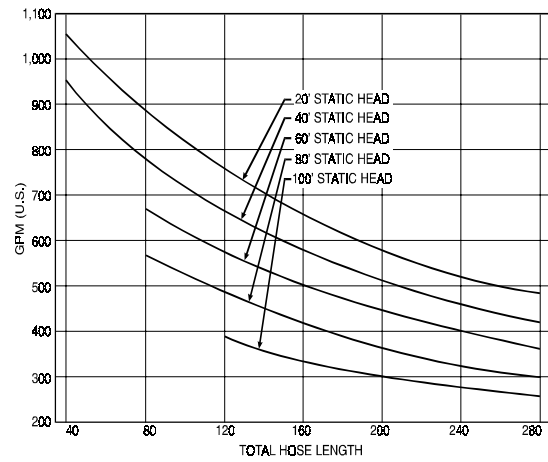
Figure 7-4M. Performance Curve, (Warm #6) CCN-150 Pump (6" Hose).
