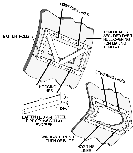
Figure 5-5. Hole Measuring Techniques and Device.
