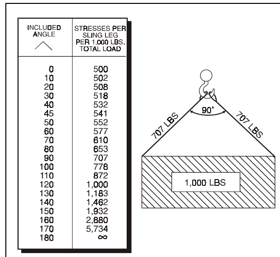
Figure 3-12. Sling Load Tension with Angular Loading.
