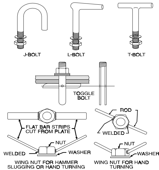
Figure 5-6. Patch Fasteners.
