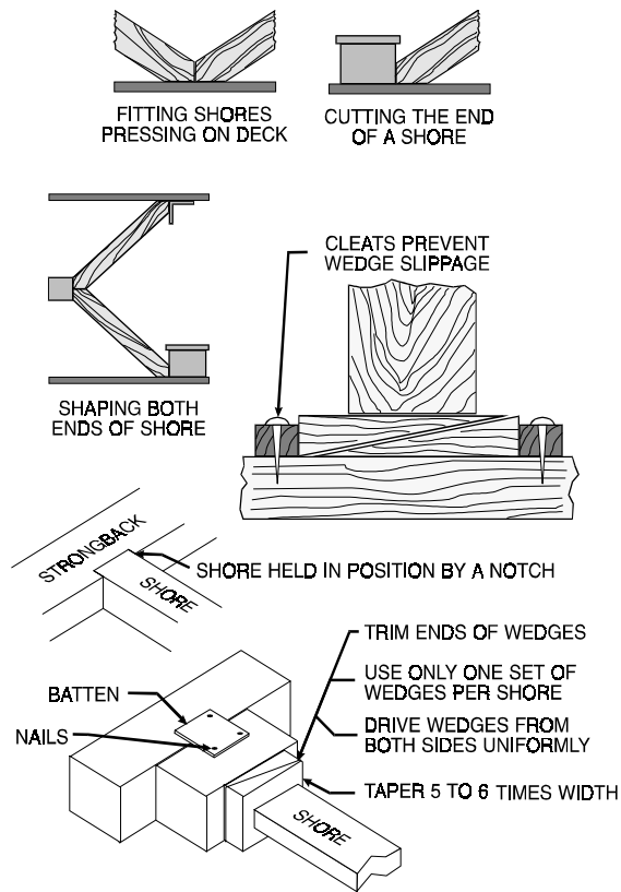
Figure 5-14. Anchoring Shores.
