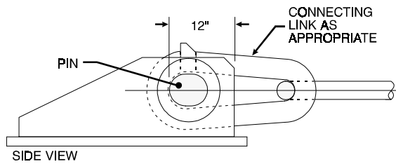
Figure 6-1. Smit Towing Bracket.
