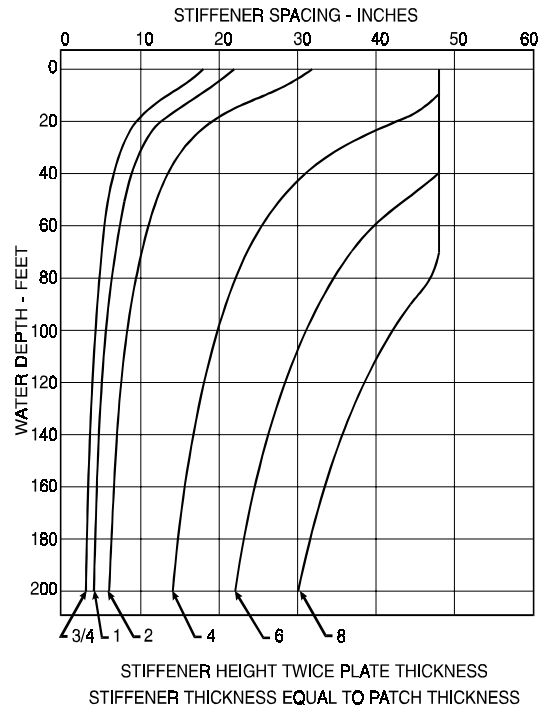
Figure 5-2B. Wood Patch Stiffener Spacing.
