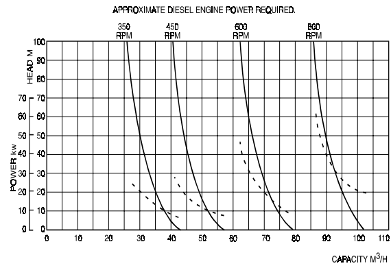
Figure 7-4P. Performance Curve, (Water) DOP-250 Pump.
