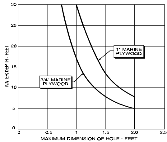
Figure 5-3. Plywood Patch Thickness.
