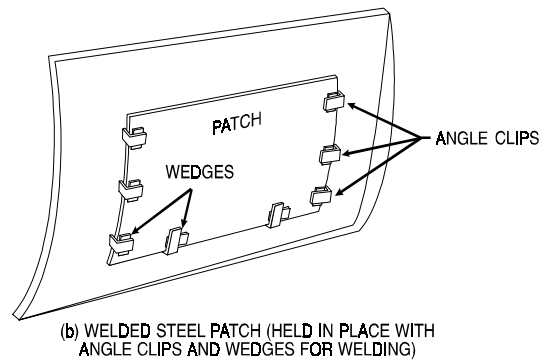
Figure 5-7. Bolted and Welded Steel Plate Patch.
