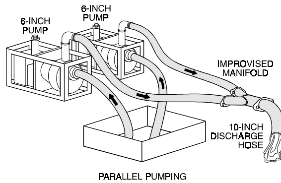
Figure 5-19B. Pumping Arrangements.
