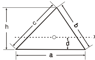
Figure 7-2A. Properties of Plane Surfaces.
