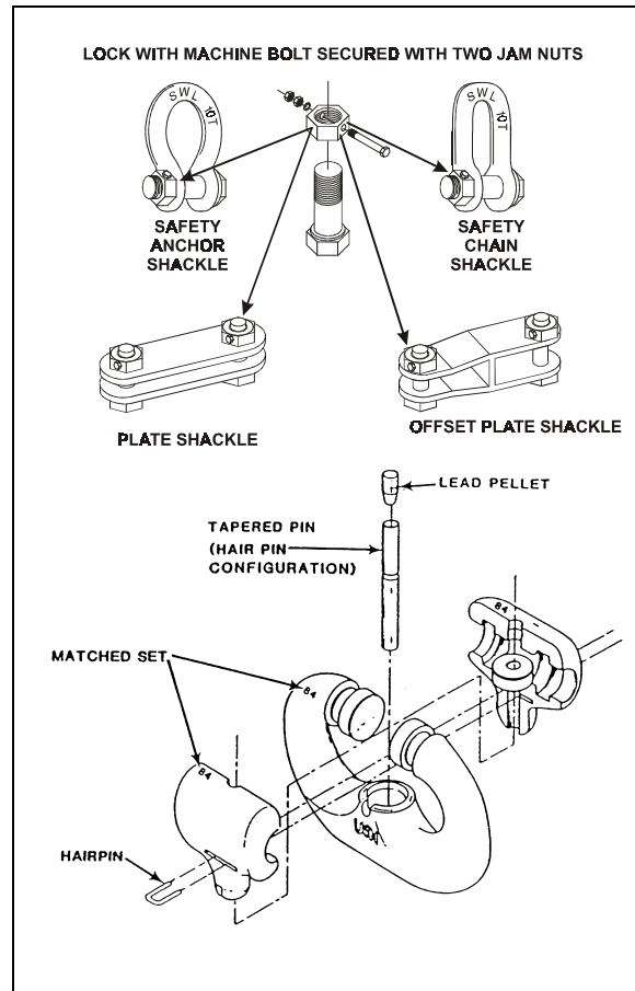
Figure 3-8. Chain Connecting Hardware
