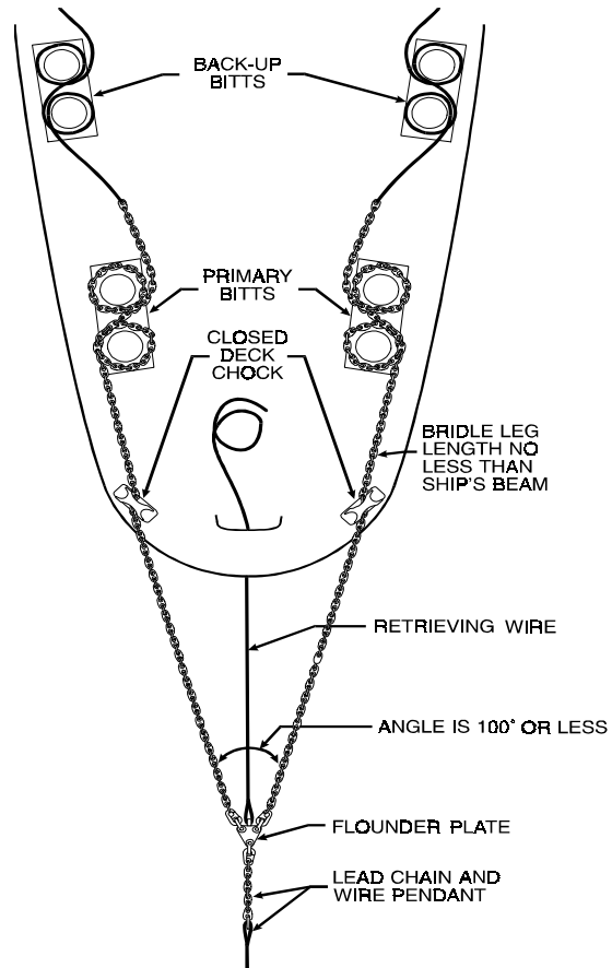
Figure 6-6A. Chain Bridle or Double Rig.
