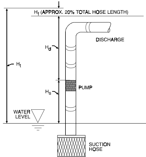
Figure 5-17. Pumping Heads.
