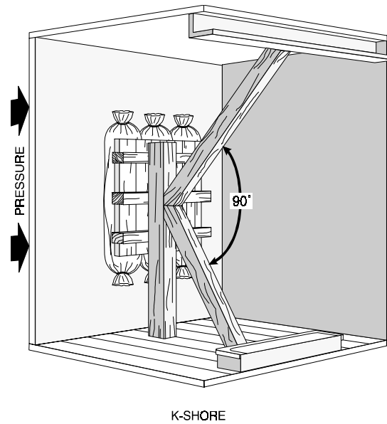
Figure 5-15. Shoring to Resist Hydrostatic Pressure.
