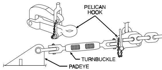
Figure 6-2. Chain Stopper.
