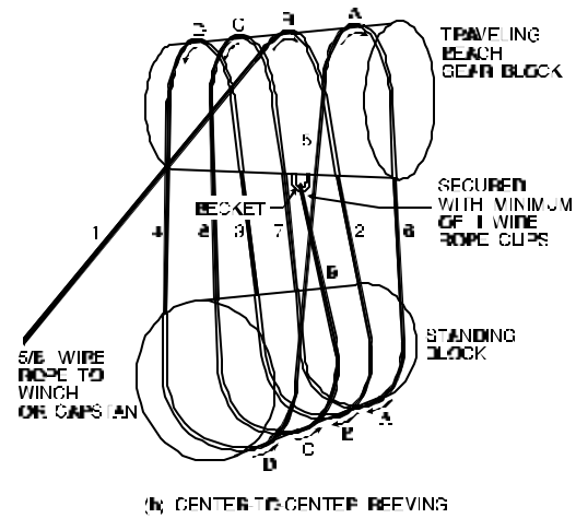
Figure 4-4. Reeving Blocks.
