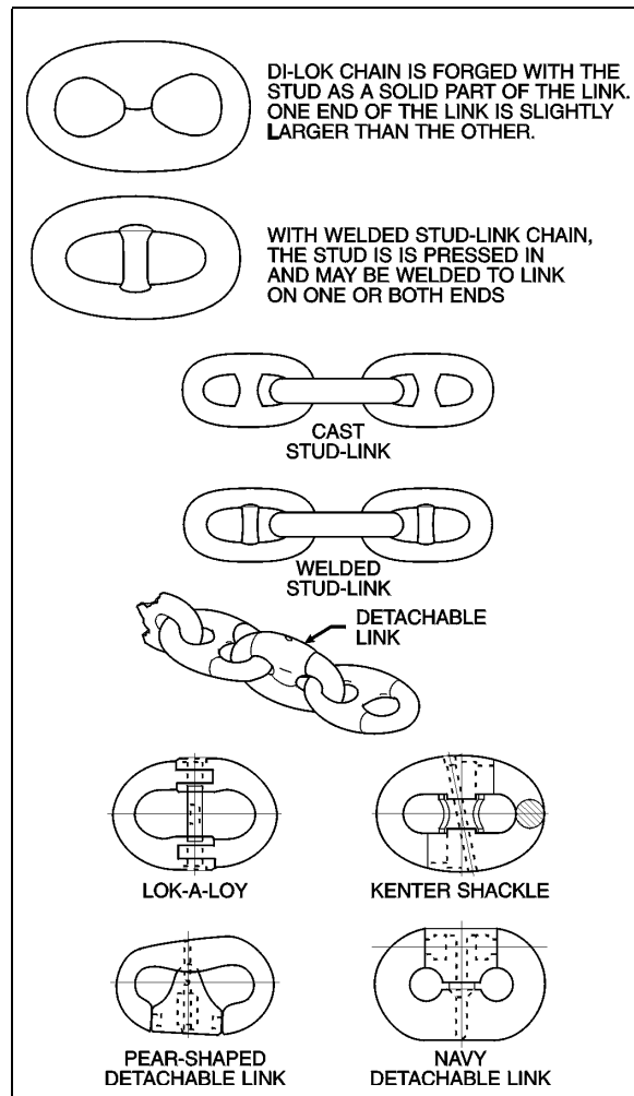
Figure 3-7. Identifying Chain and Fittings.
