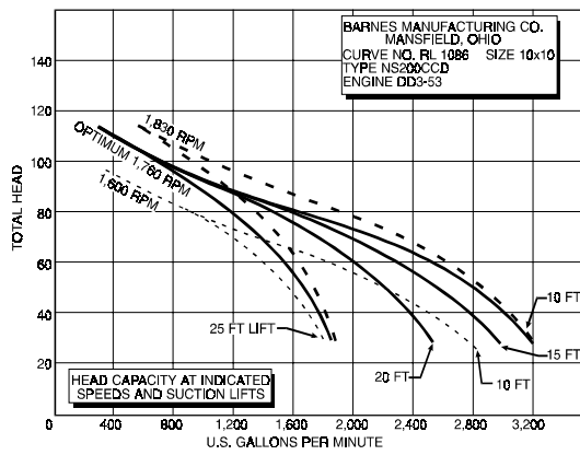
Figure 7-4C. Performance Curve, 10-inch Diesel Pump.
