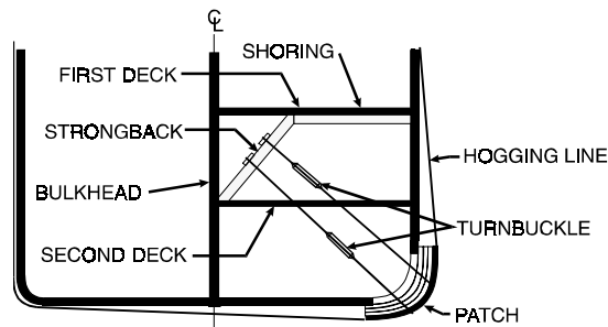
Figure 5-8. Patch Secured with Turnbuckle and Strongback.
