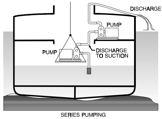
Figure 5-19A. Pumping Arrangements.
