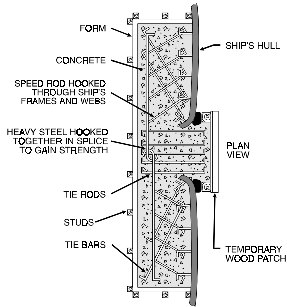
Figure 5-11. Large Reinforced Concrete Patch.
