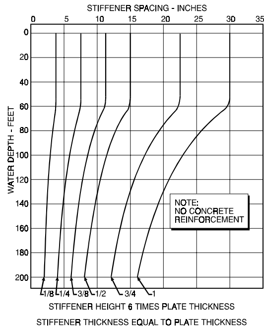
Figure 5-2A. Steel Patch Stiffener Spacing.
