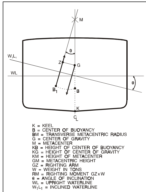
Figure 2-1. Centers, Heights and Righting Arm.
