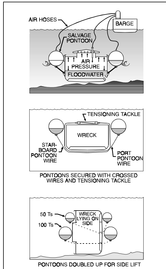
Figure 3-14. Rigging Pontoons and Lift Bags.
