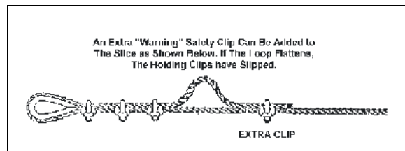
Figure 3-5. Joining Wire Ropes.
